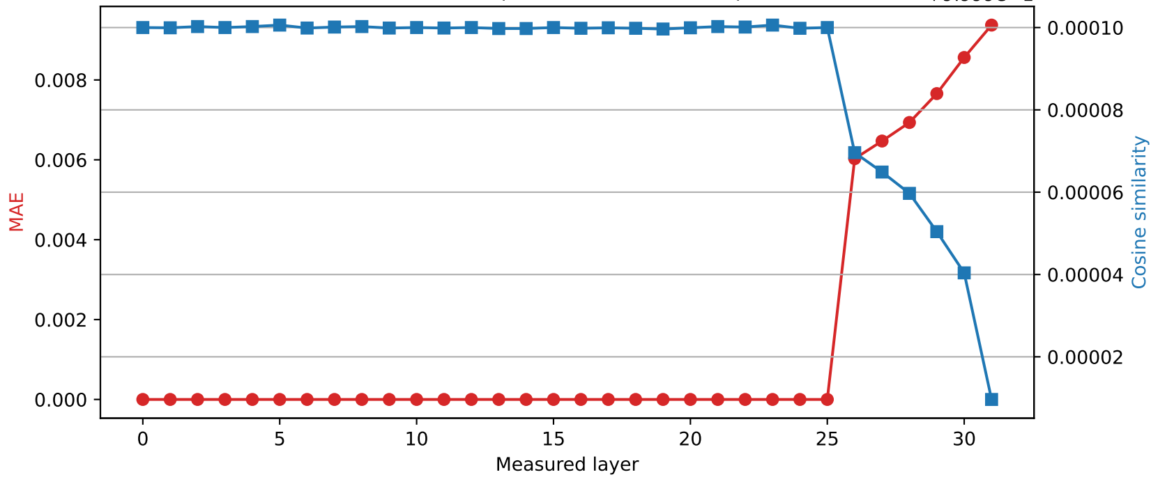
Mistral-7B-Instruct-v0.3 | Quantized layer 25 | float16 \rightarrow int8 +9.999e-1
