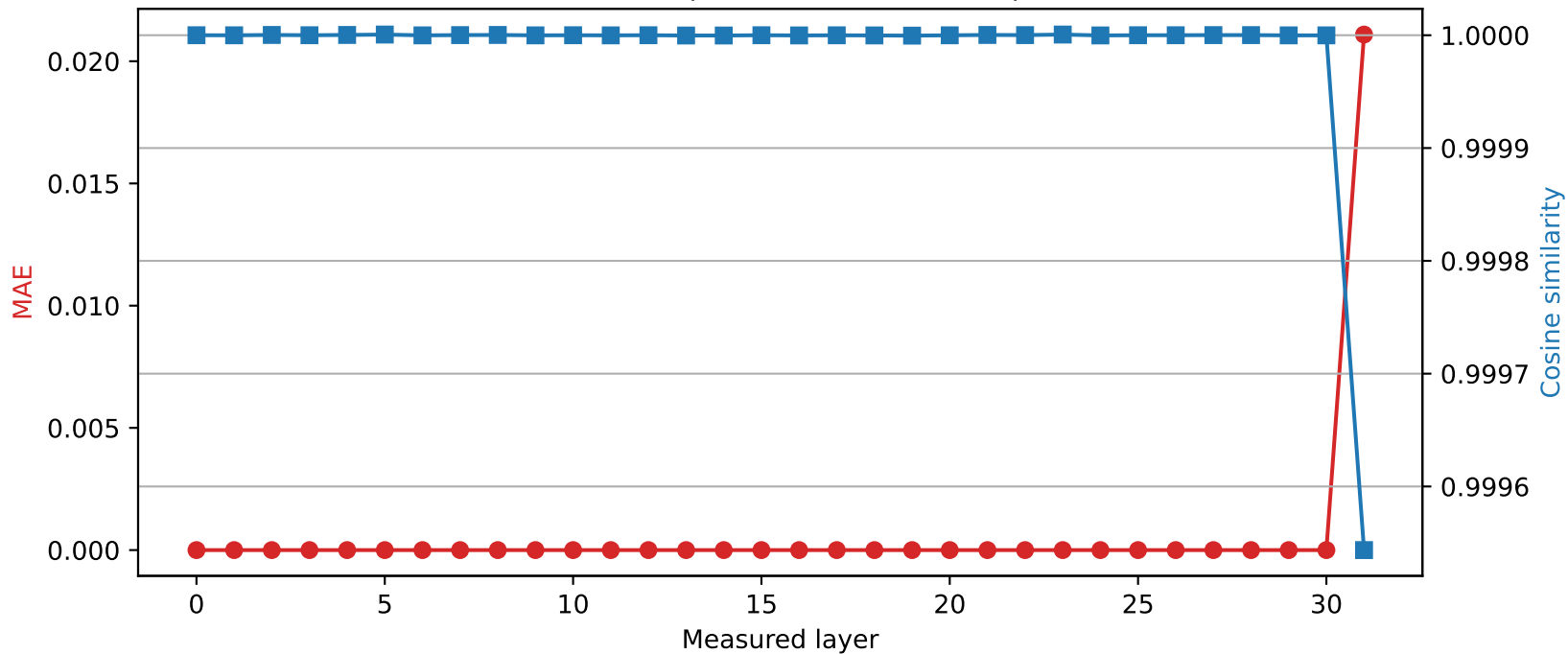
Mistral-7B-Instruct-v0.3 | Quantized layer 30 | float16 \rightarrow int8
