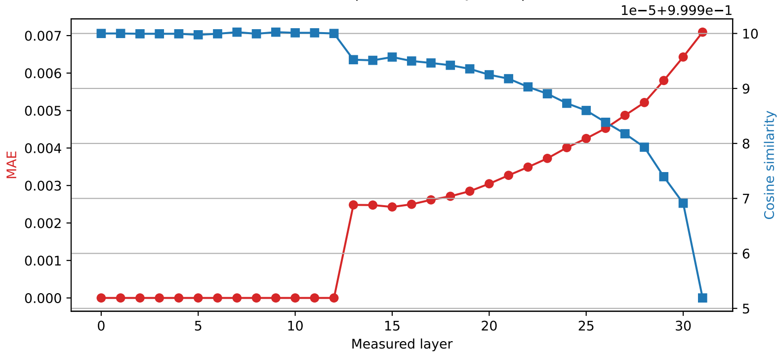
Mistral-7B-Instruct-v0.3 | Quantized layer 12 | float16 → int8
