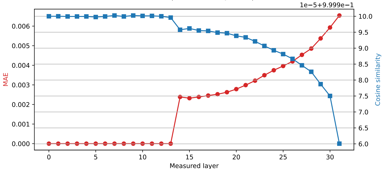
Mistral-7B-Instruct-v0.3 | Quantized layer 13 | float16 → int8
