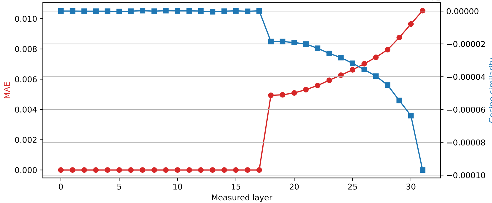
Mistral-7B-Instruct-v0.3 | Quantized layer 17 | float16 \rightarrow int8
