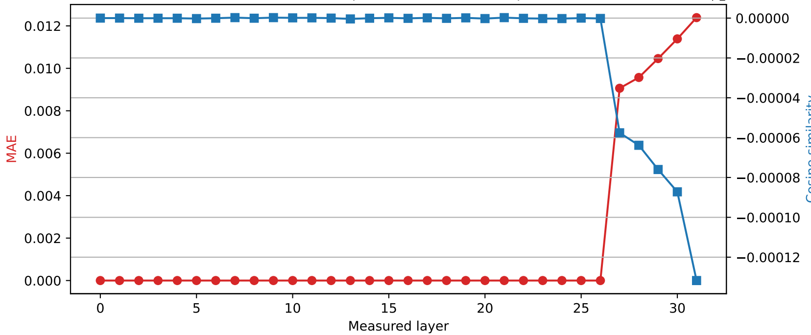
Mistral-7B-Instruct-v0.3 | Quantized layer 26 | float16 \rightarrow int8
