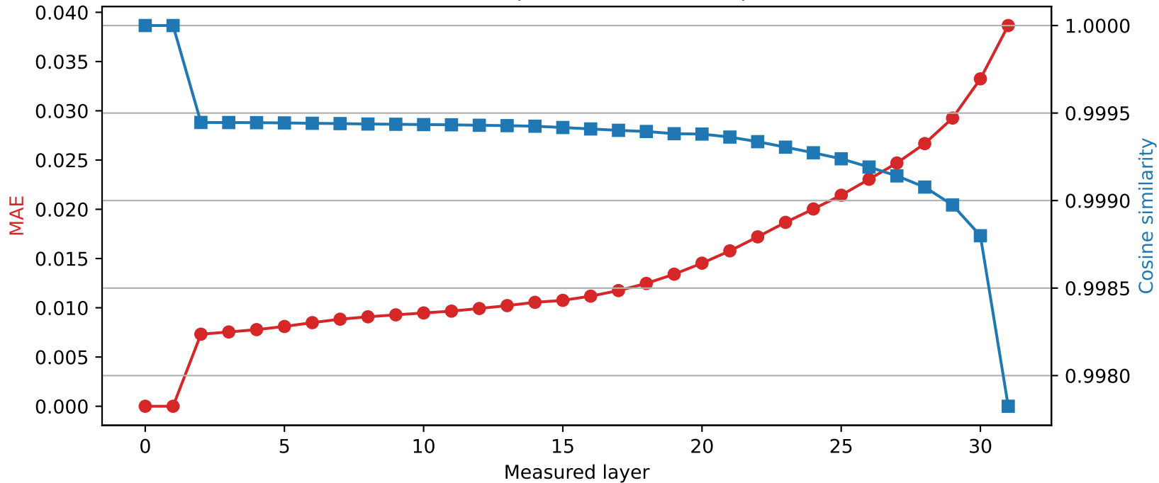
Mistral-7B-Instruct-v0.3 | Quantized layer 1 | float16 → int8
