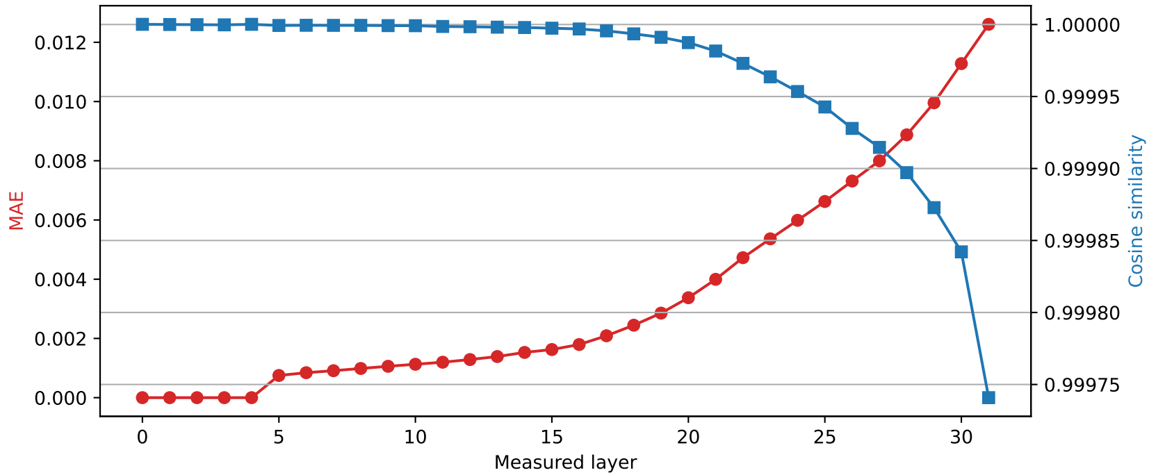
Mistral-7B-Instruct-v0.3 | Quantized layer 4 | float16 → int8
