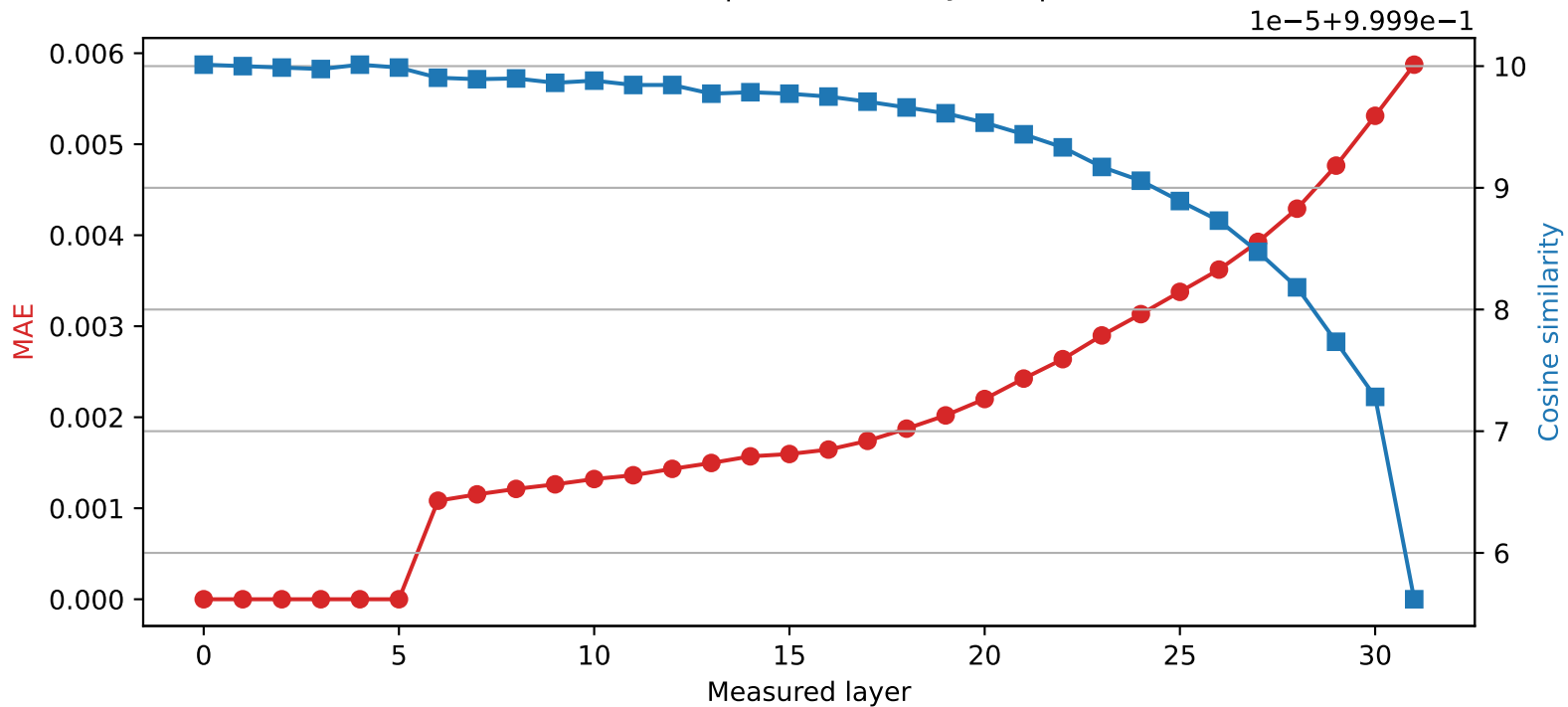
Mistral-7B-Instruct-v0.3 | Quantized layer 5 | float16 → int8
