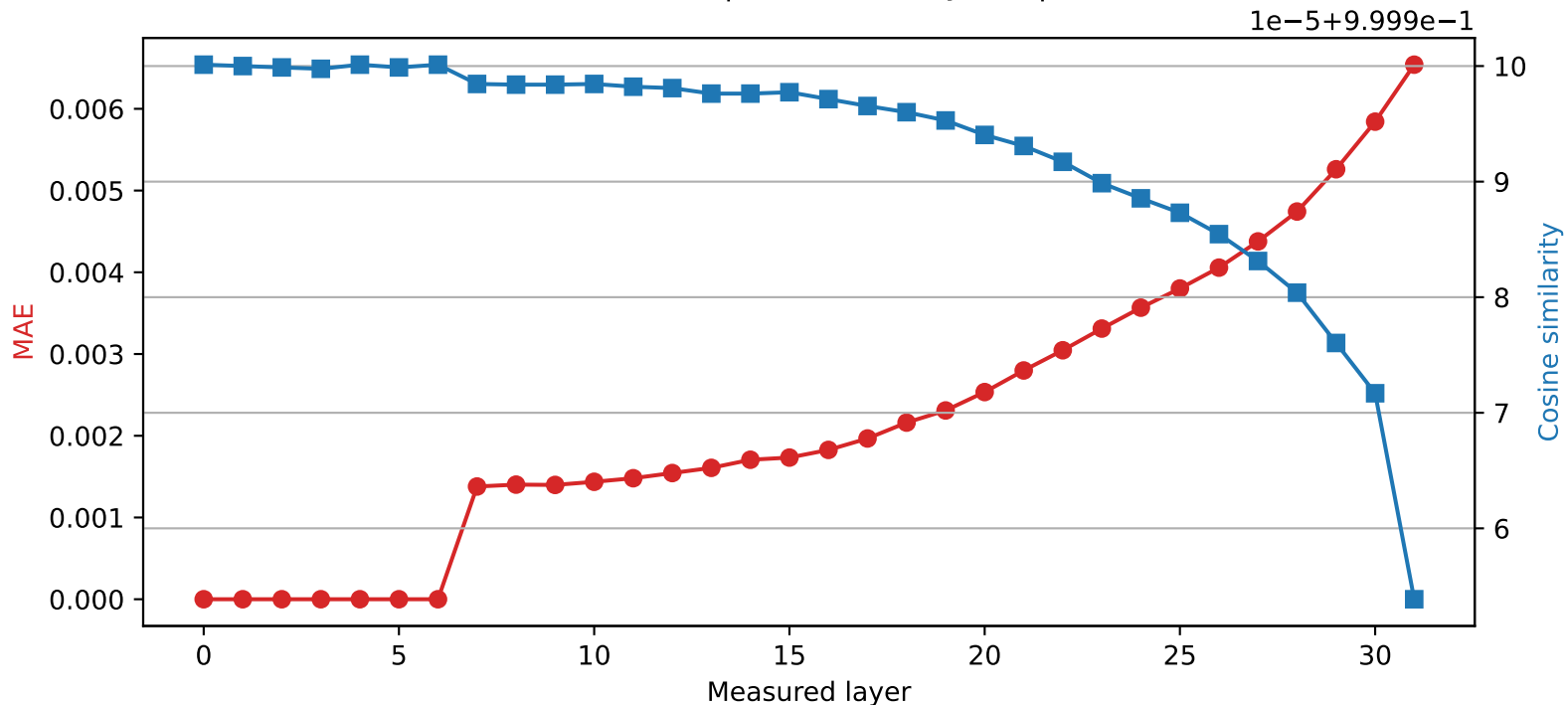
Mistral-7B-Instruct-v0.3 | Quantized layer 6 | float16 → int8
