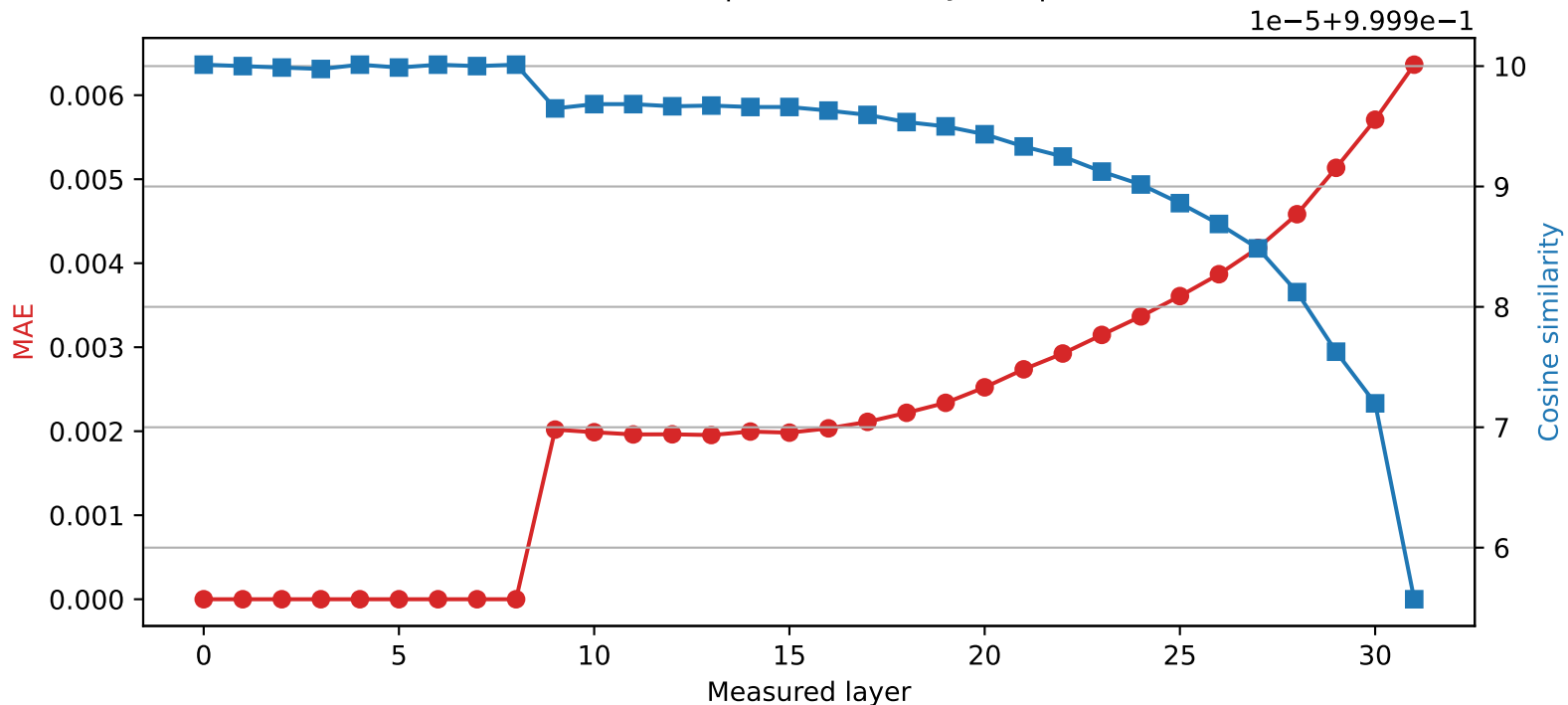
Mistral-7B-Instruct-v0.3 | Quantized layer 8 | float16 → int8
