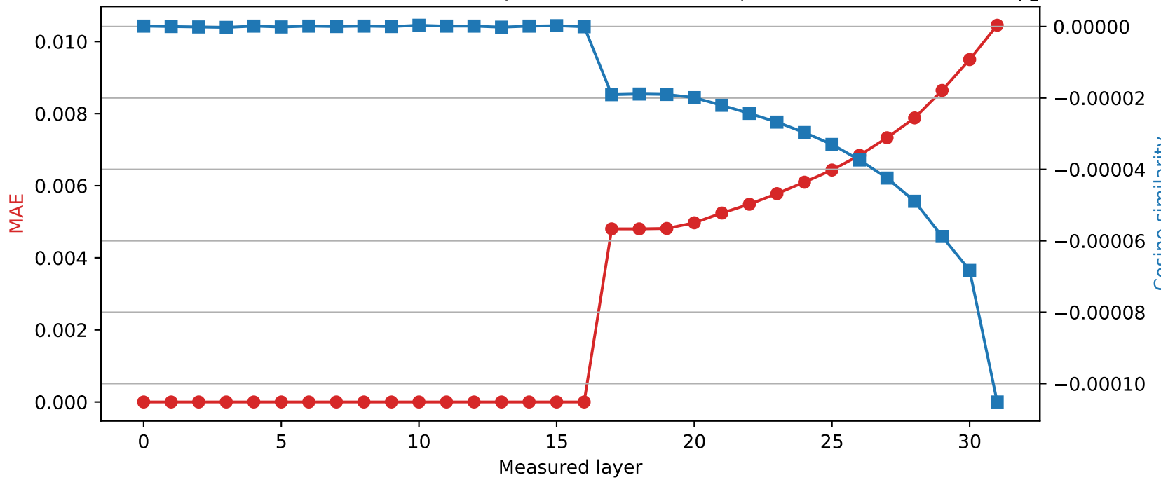
Mistral-7B-Instruct-v0.3 | Quantized layer 16 | float16 \rightarrow int8
