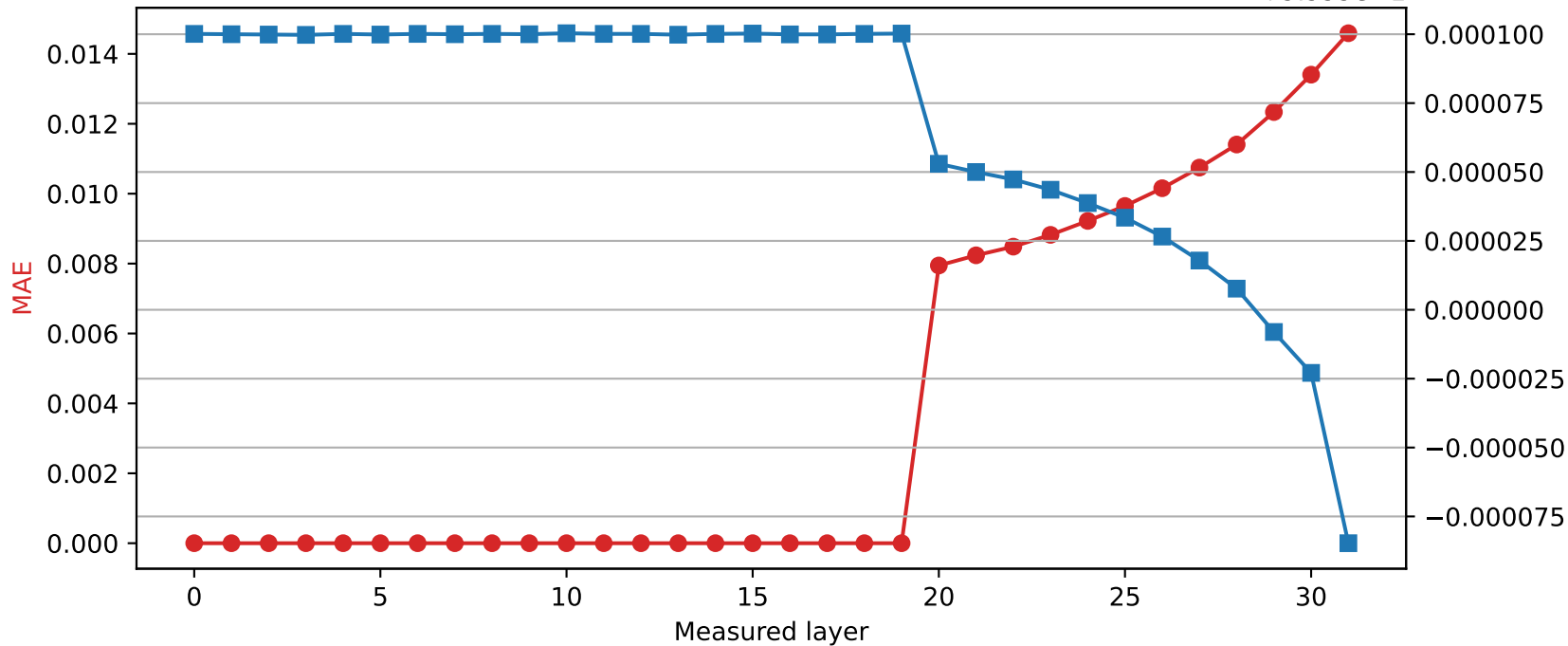
Mistral-7B-Instruct-v0.3 | Quantized layer 19 | float16 \rightarrow int8 +9.999e-1
