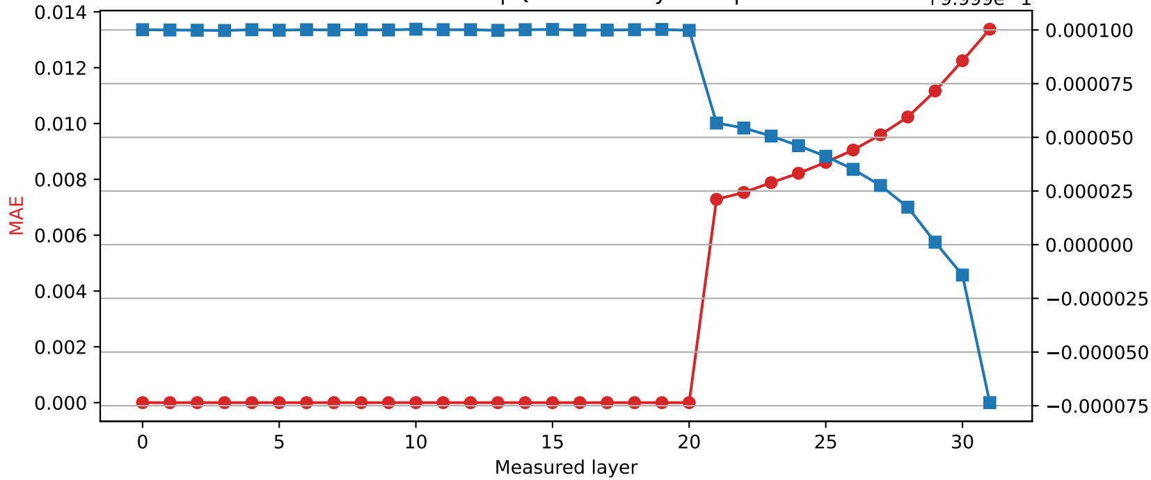
Mistral-7B-Instruct-v0.3 | Quantized layer 20 | float16 \rightarrow int8 +9.999e-1
