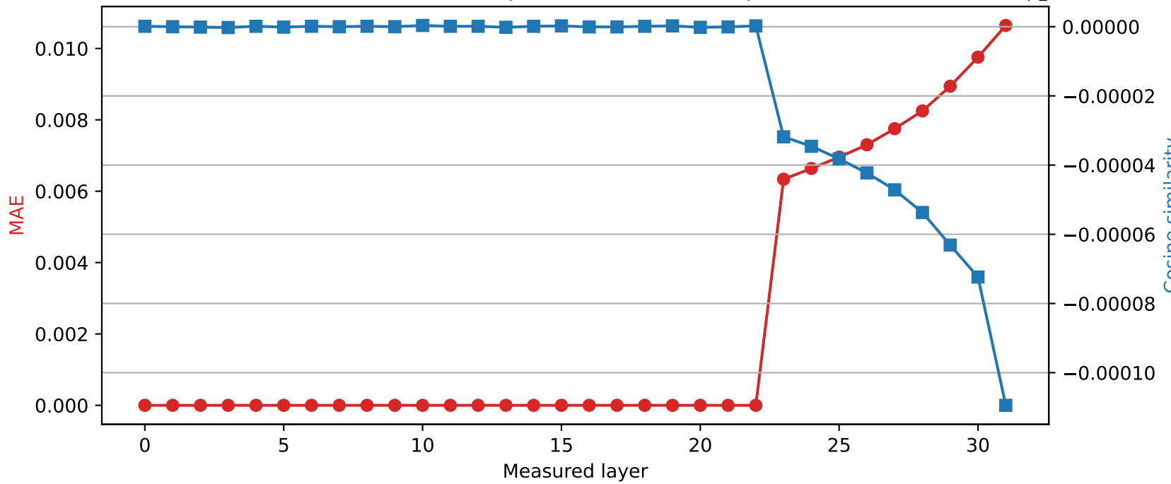
Mistral-7B-Instruct-v0.3 | Quantized layer 22 | float16 \rightarrow int8
