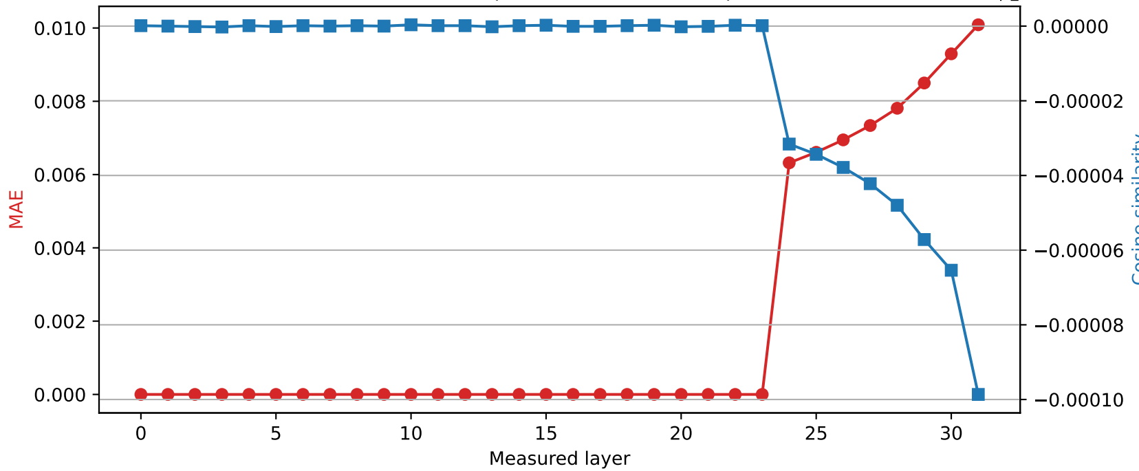
Mistral-7B-Instruct-v0.3 | Quantized layer 23 | float16 \rightarrow int8
