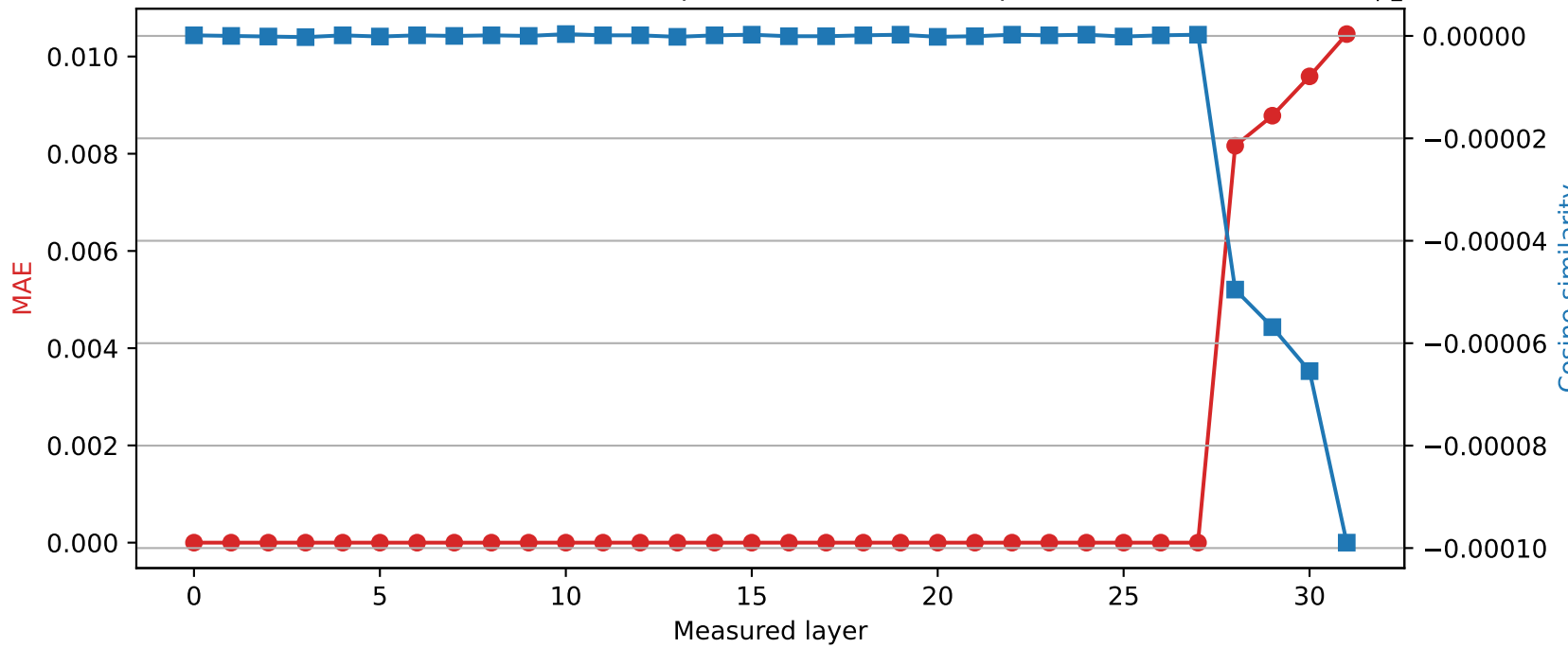
Mistral-7B-Instruct-v0.3 | Quantized layer 27 | float16 \rightarrow int8
