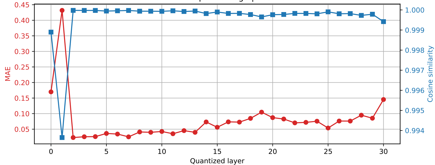
Mistral-7B-Instruct-v0.3 | Prompt 4 Final RMSNorm output damage | float16 \rightarrow int8
