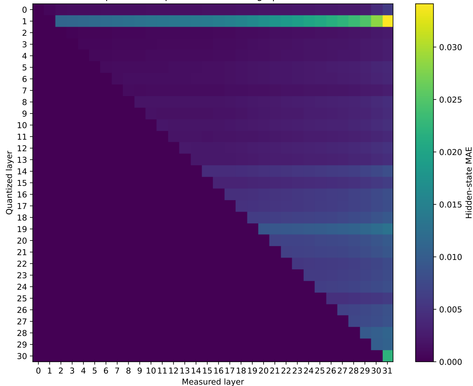
Mistral-7B-Instruct-v0.3 Prompt 4: MAE representation damage | float16 \rightarrow int8
