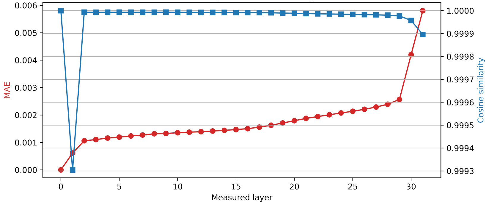
Mistral-7B-Instruct-v0.3 | Quantized layer 0 | float16 \rightarrow int8
