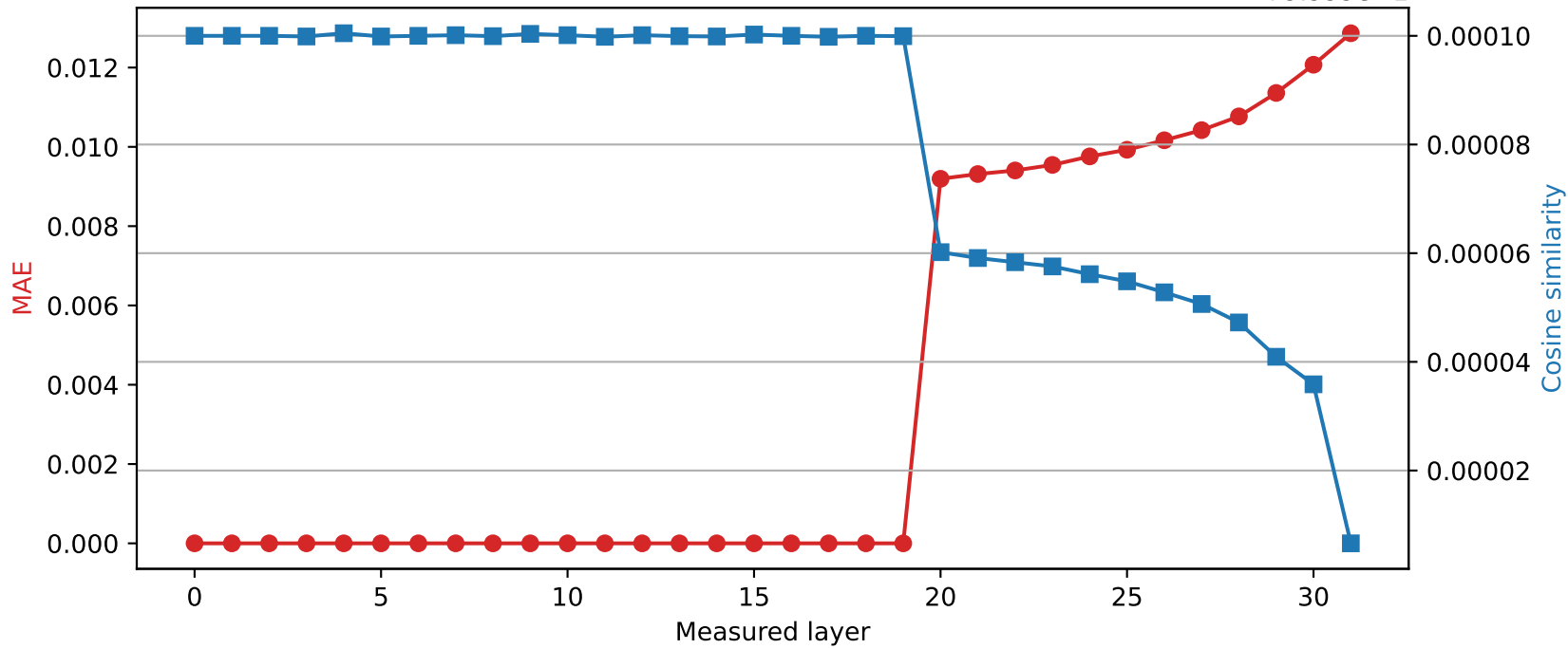
Mistral-7B-Instruct-v0.3 | Quantized layer 19 | float16 → int8 +9.999e-1
