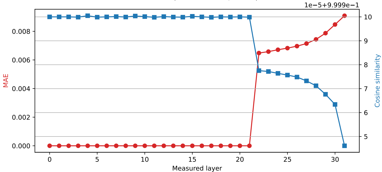
Mistral-7B-Instruct-v0.3 | Quantized layer 21 | float16 \rightarrow int8
