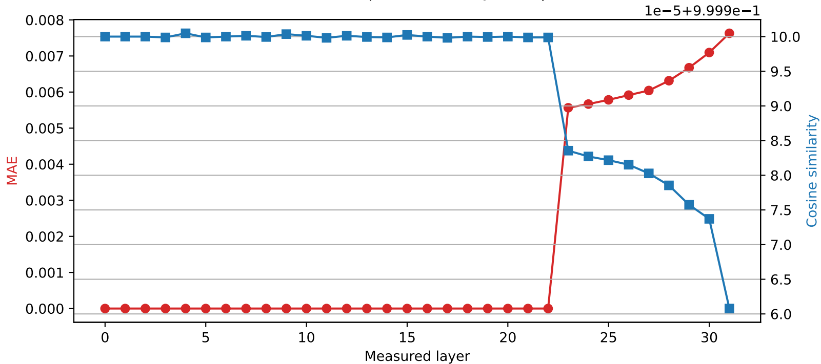
Mistral-7B-Instruct-v0.3 | Quantized layer 22 | float16 → int8
