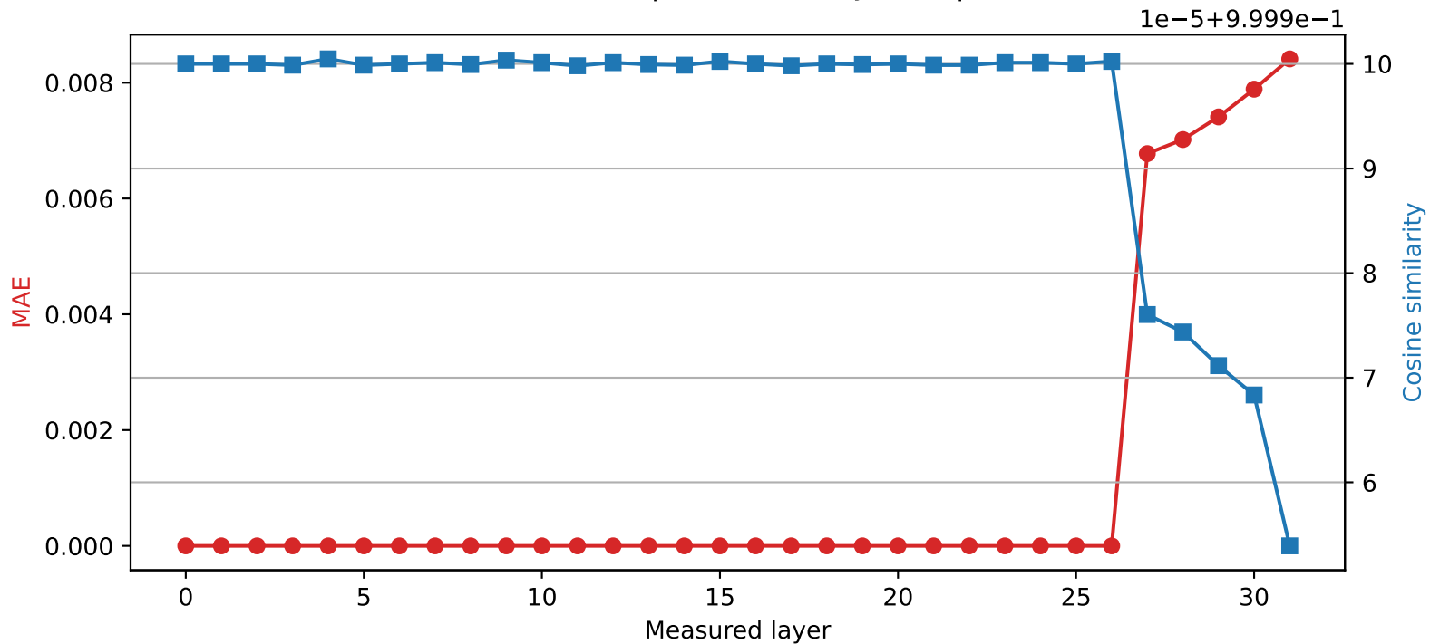
Mistral-7B-Instruct-v0.3 | Quantized layer 26 | float16 \rightarrow int8
