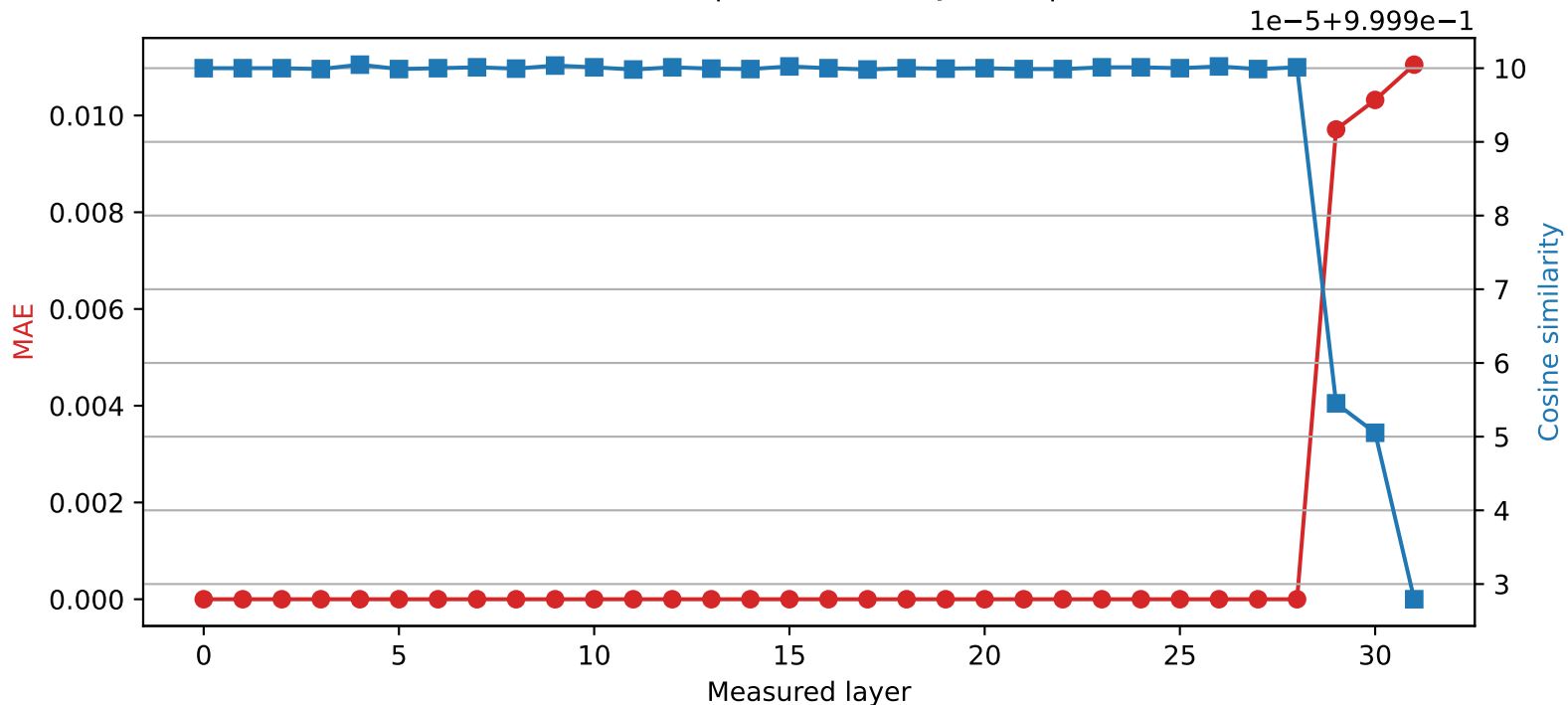
Mistral-7B-Instruct-v0.3 | Quantized layer 28 | float16 → int8
