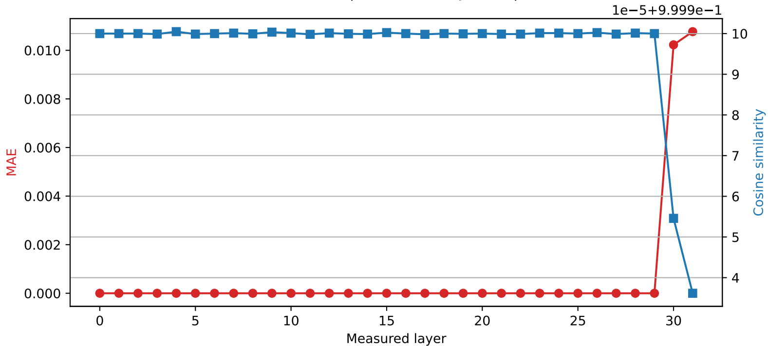
Mistral-7B-Instruct-v0.3 | Quantized layer 29 | float16 \rightarrow int8
