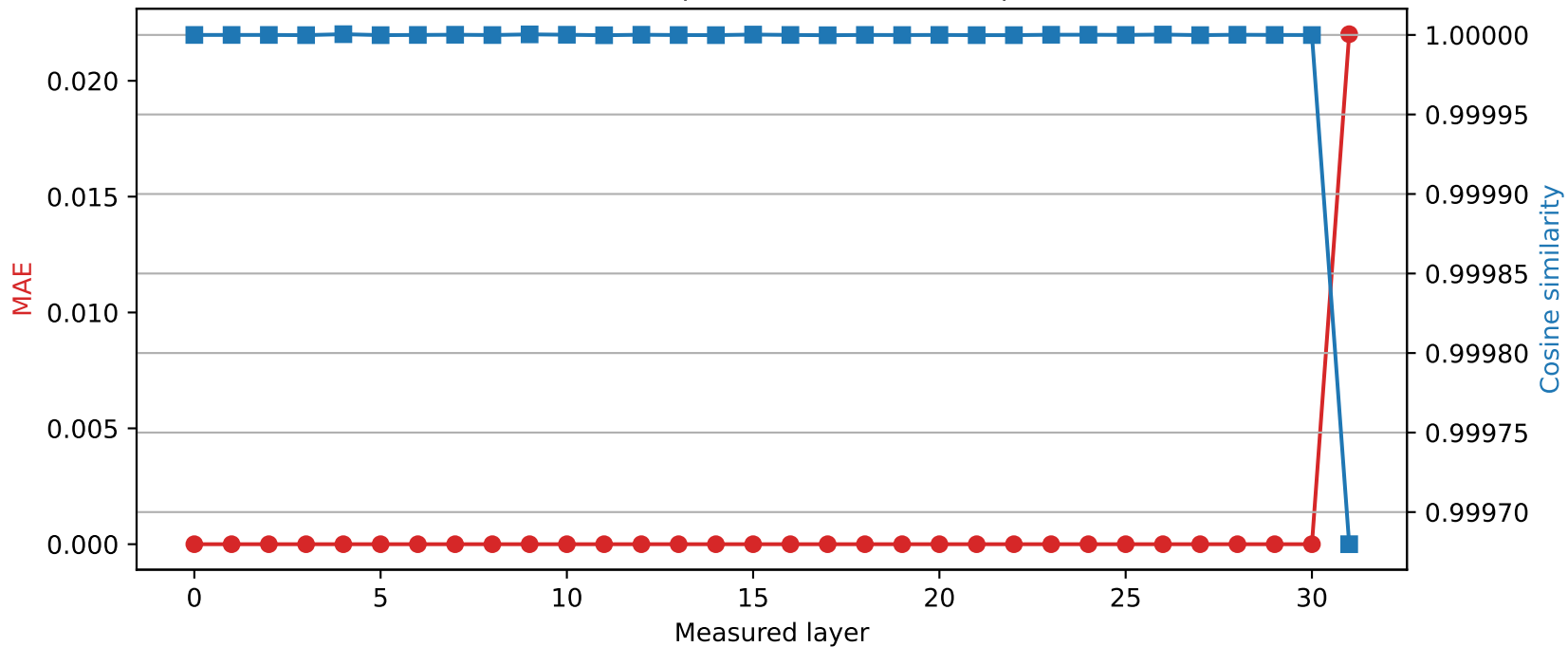
Mistral-7B-Instruct-v0.3 | Quantized layer 30 | float16 \rightarrow int8
