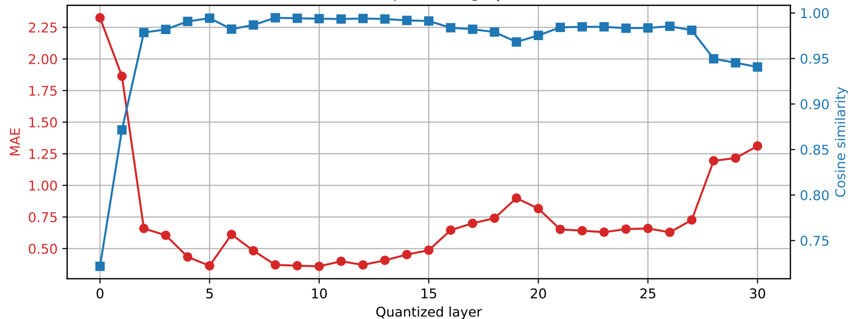
Mistral-7B-Instruct-v0.3 | Prompt 0 Final RMSNorm output damage | float16 \rightarrow int4
