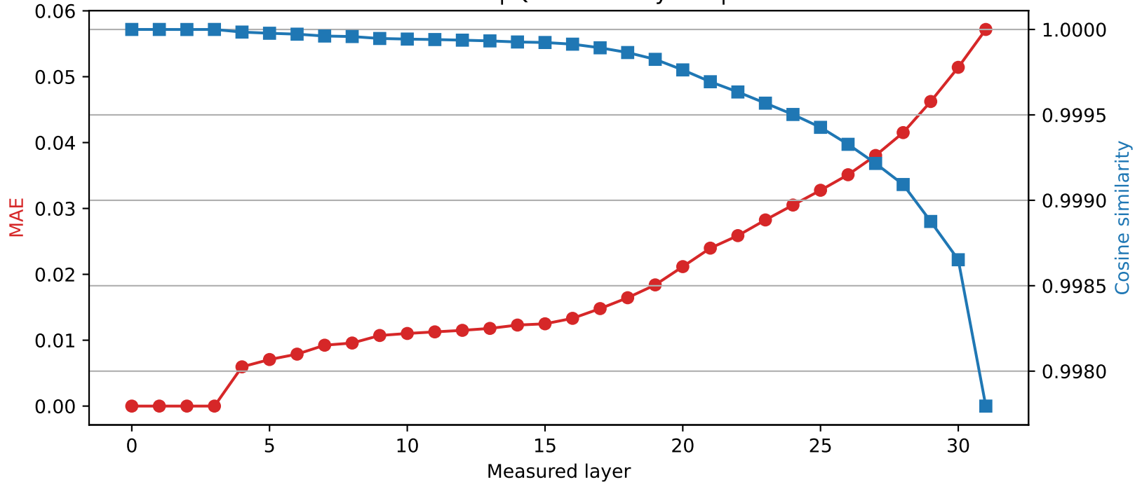
Mistral-7B-Instruct-v0.3 | Quantized layer 3 | float16 \rightarrow int4
