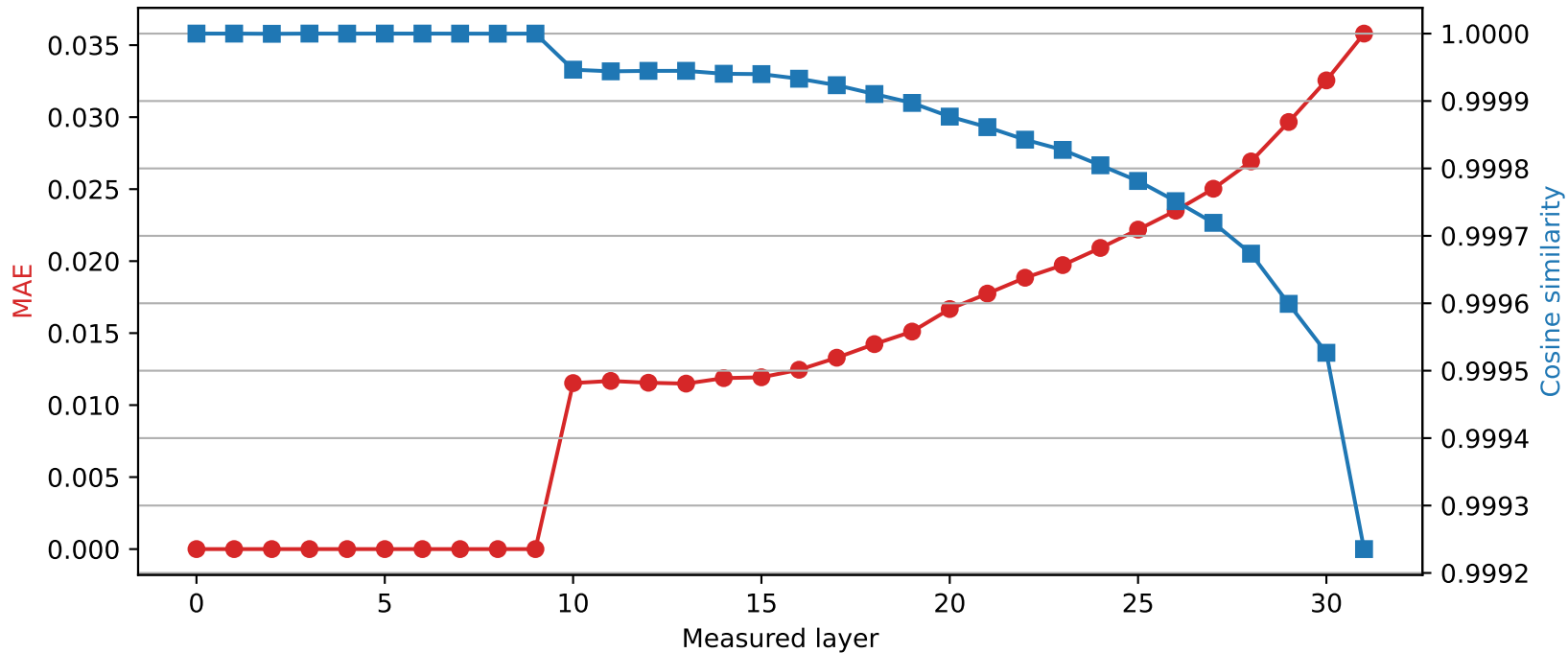
Mistral-7B-Instruct-v0.3 | Quantized layer 9 | float16 \rightarrow int4
