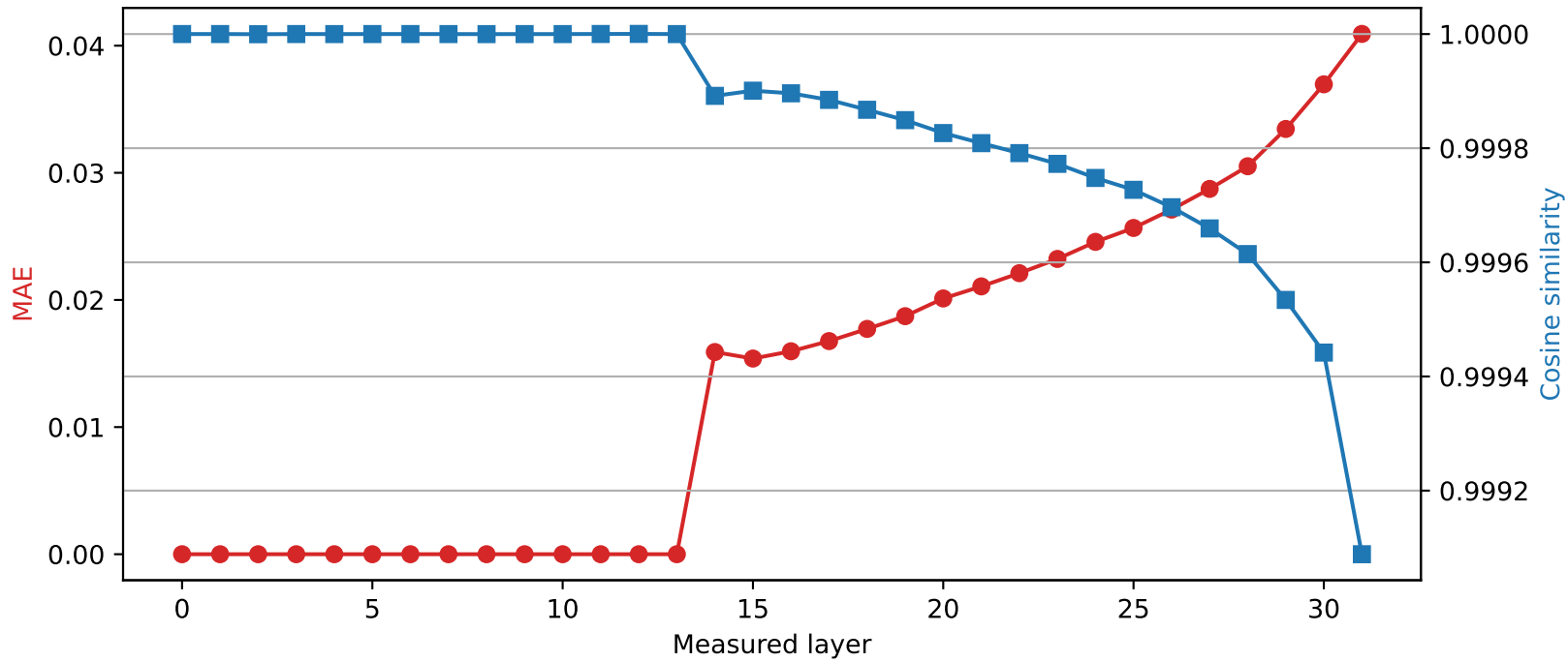
Mistral-7B-Instruct-v0.3 | Quantized layer 13 | float16 \rightarrow int4
