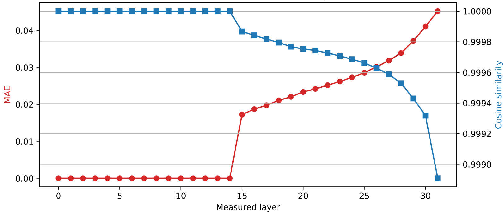
Mistral-7B-Instruct-v0.3 | Quantized layer 14 | float16 → int4
