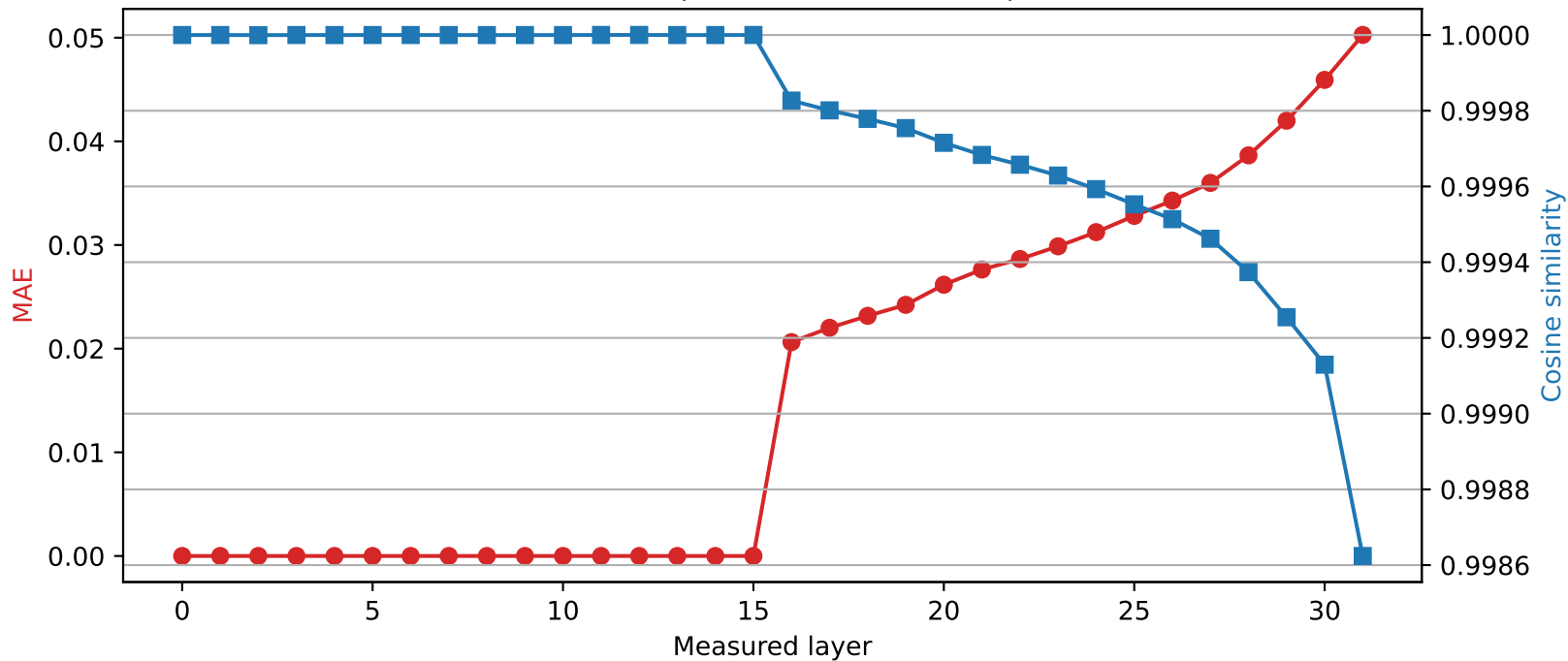
Mistral-7B-Instruct-v0.3 | Quantized layer 15 | float16 \rightarrow int4
