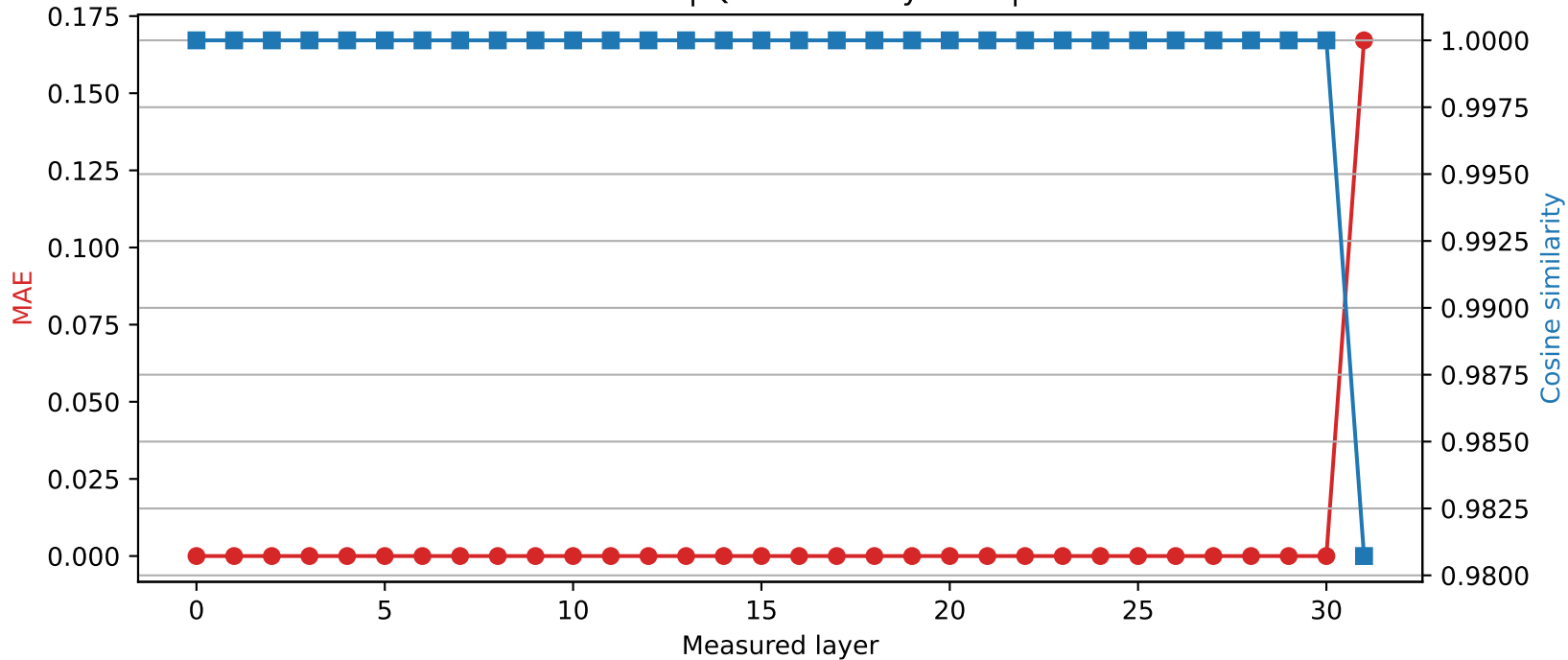
Mistral-7B-Instruct-v0.3 | Quantized layer 30 | float16 \rightarrow int4
