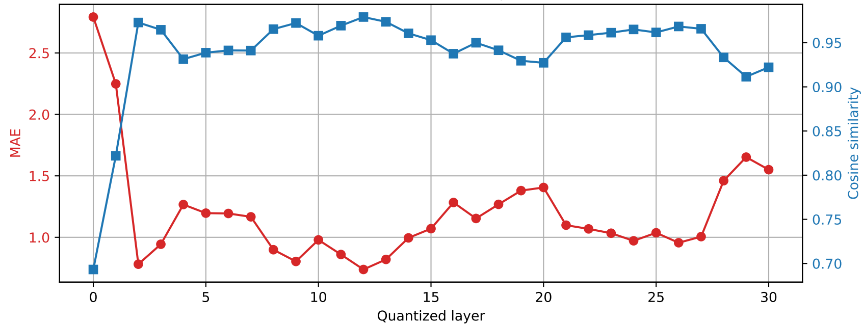
Mistral-7B-Instruct-v0.3 | Prompt 1 Final RMSNorm output damage | float16 \rightarrow int4
