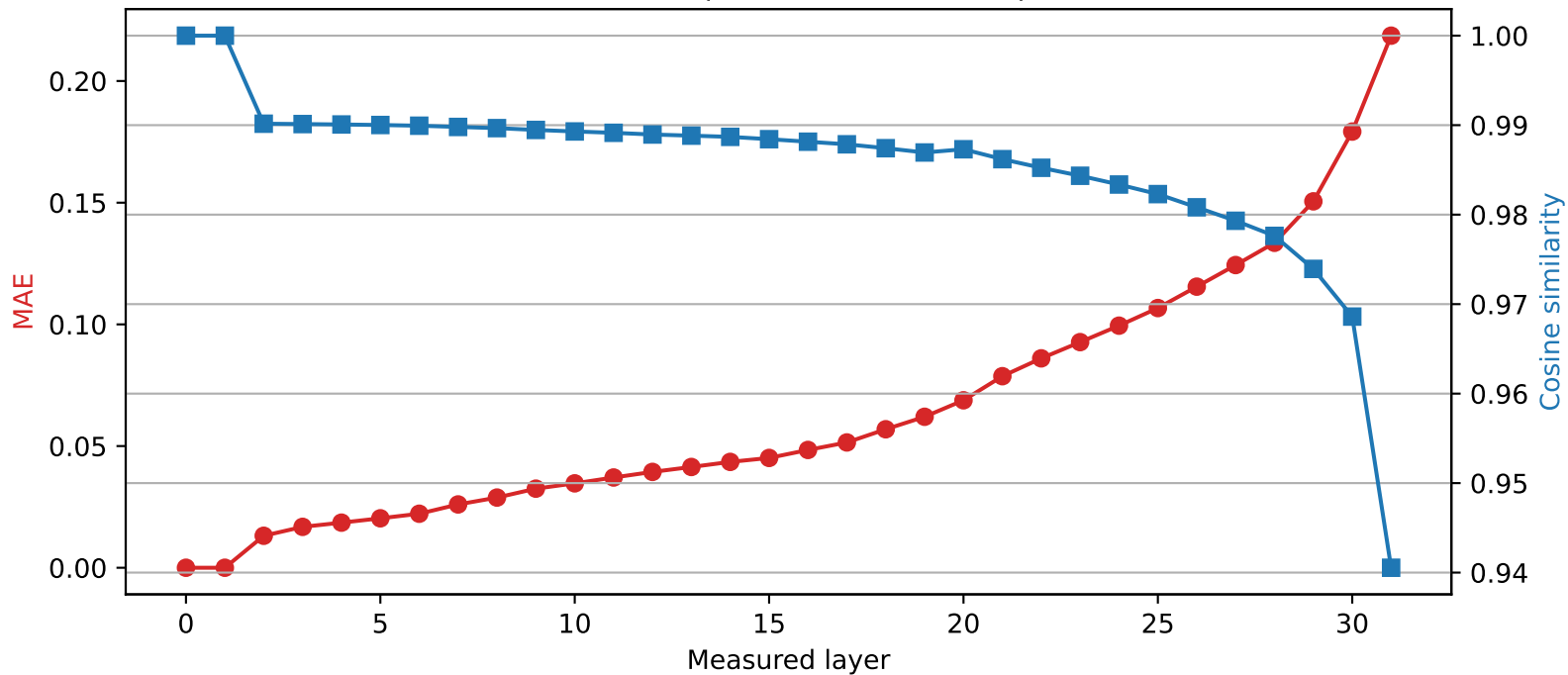
Mistral-7B-Instruct-v0.3 | Quantized layer 1 | float16 \rightarrow int4
