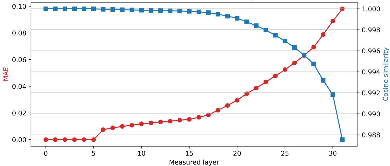
Mistral-7B-Instruct-v0.3 | Quantized layer 5 | float16 → int4
