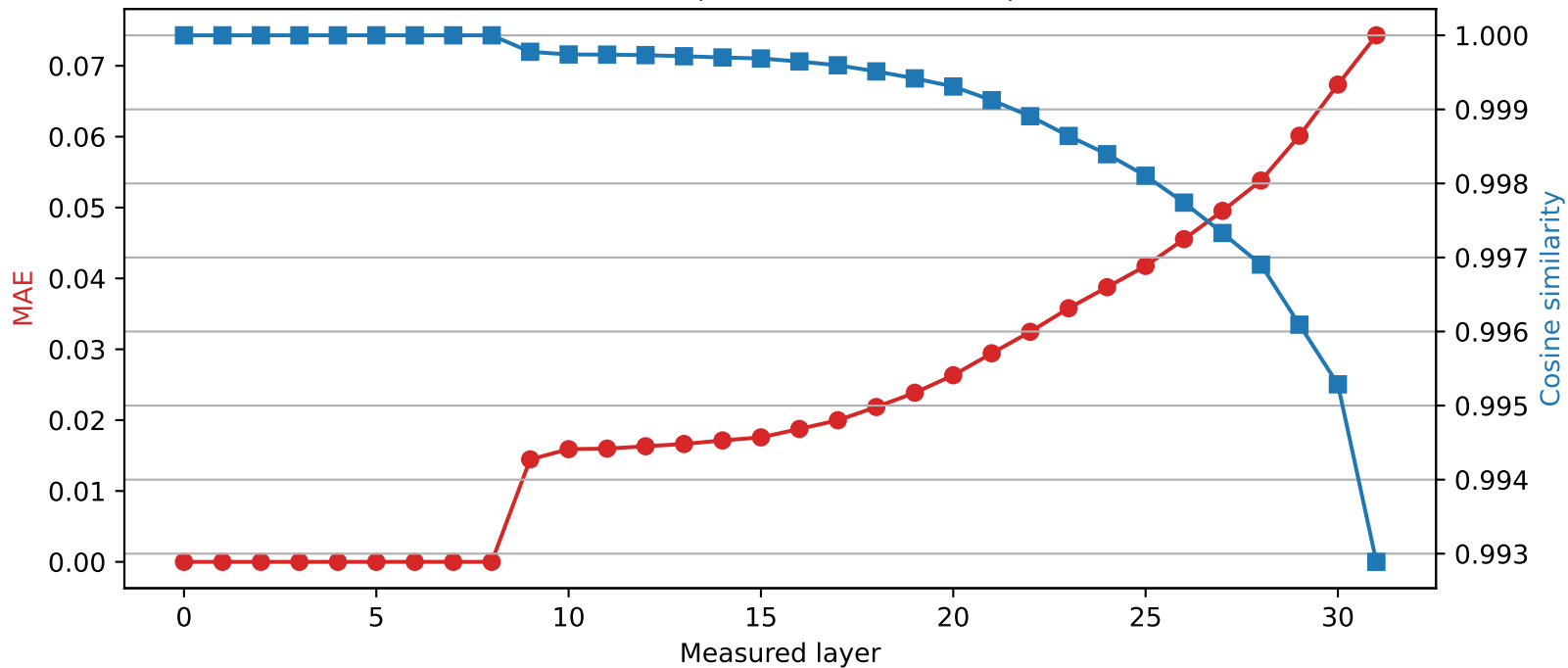
Mistral-7B-Instruct-v0.3 | Quantized layer 8 | float16 → int4
