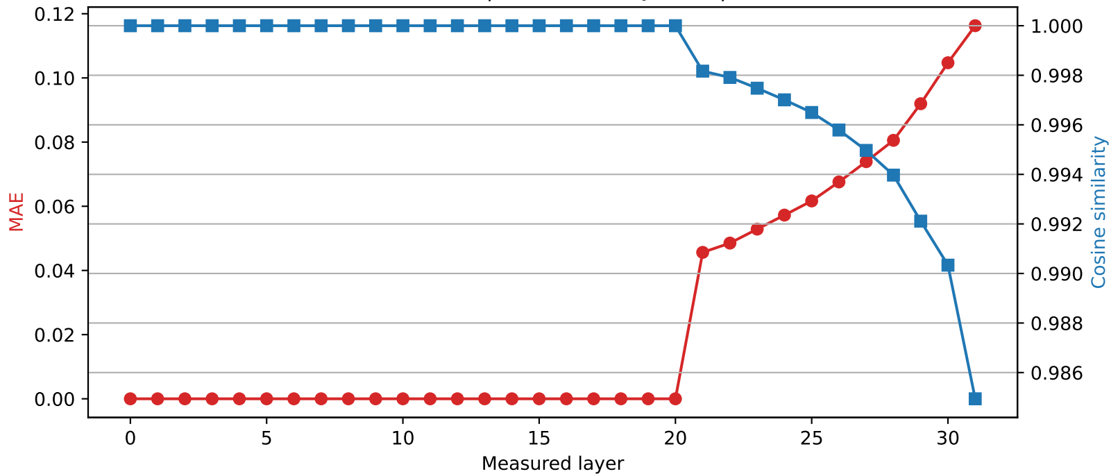
Mistral-7B-Instruct-v0.3 | Quantized layer 20 | float16 \rightarrow int4
