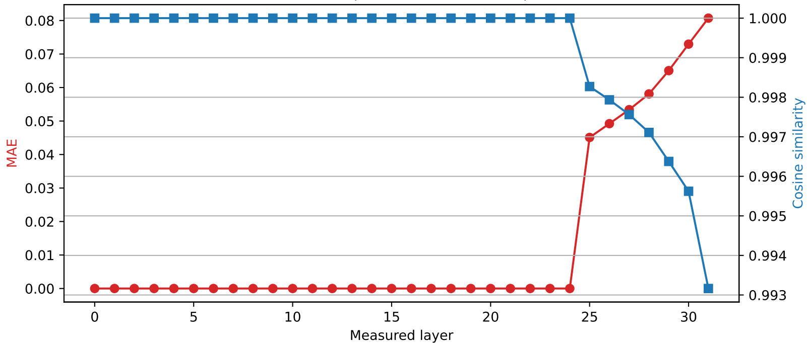
Mistral-7B-Instruct-v0.3 | Quantized layer 24 | float16 \rightarrow int4
