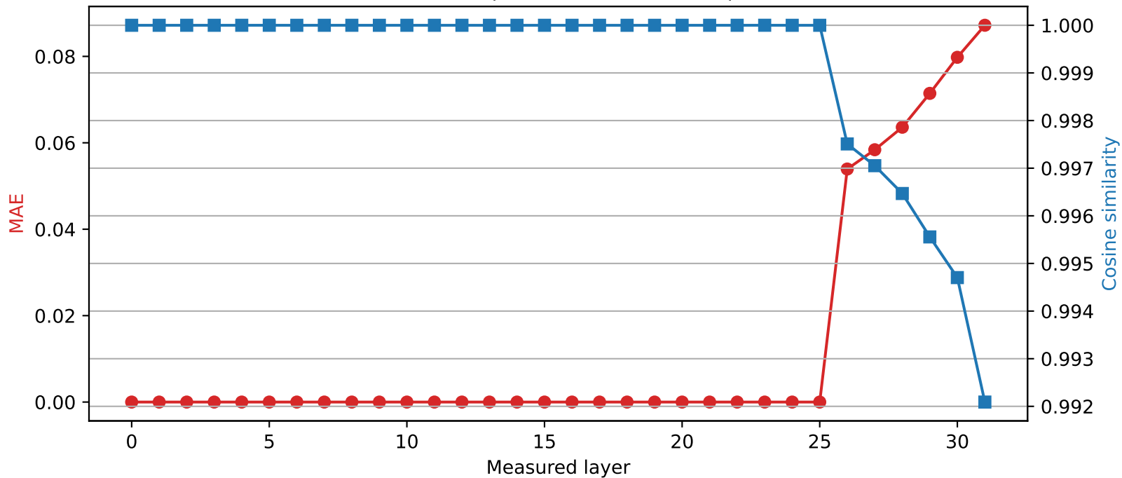
Mistral-7B-Instruct-v0.3 | Quantized layer 25 | float16 \rightarrow int4
