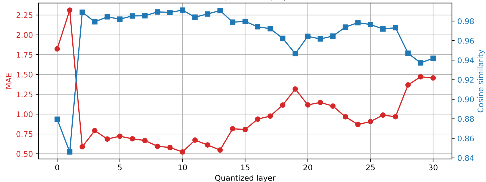
Mistral-7B-Instruct-v0.3 | Prompt 2 Final RMSNorm output damage | float16 \rightarrow int4
