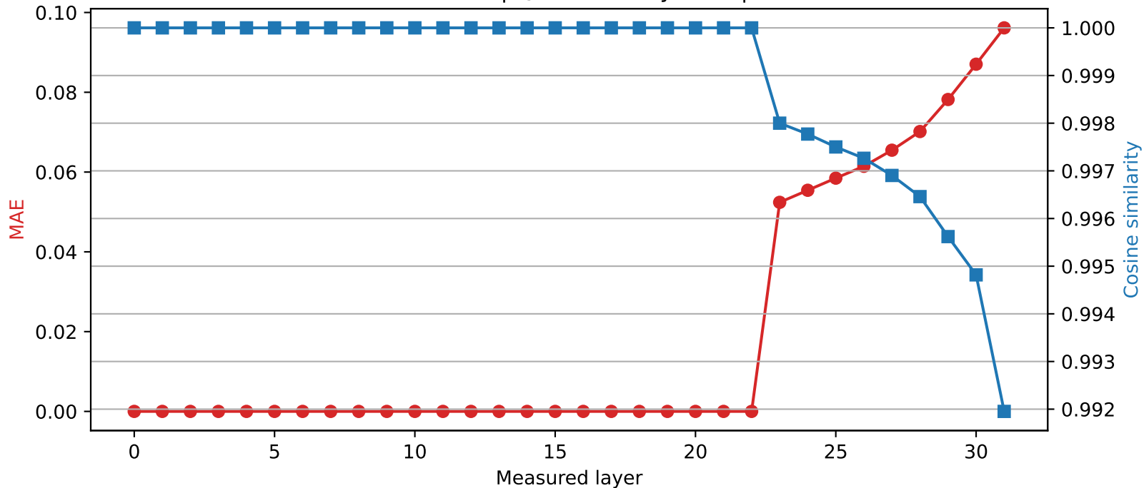
Mistral-7B-Instruct-v0.3 | Quantized layer 22 | float16 \rightarrow int4
