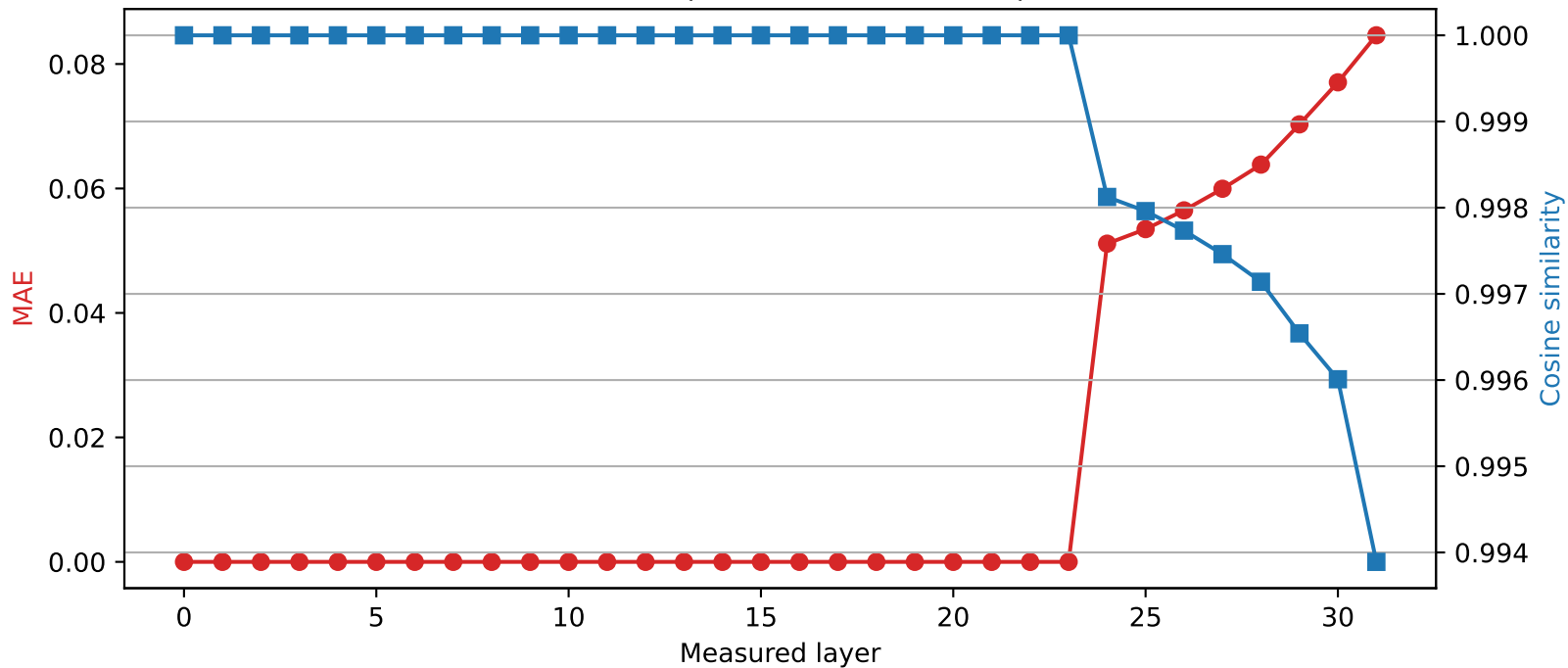
Mistral-7B-Instruct-v0.3 | Quantized layer 23 | float16 \rightarrow int4
