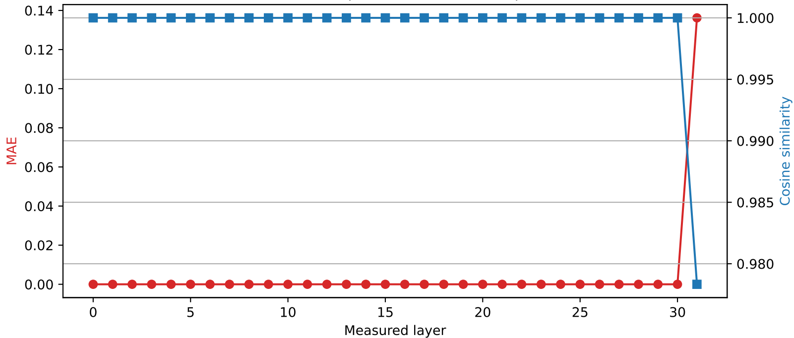
Mistral-7B-Instruct-v0.3 | Quantized layer 30 | float16 \rightarrow int4
