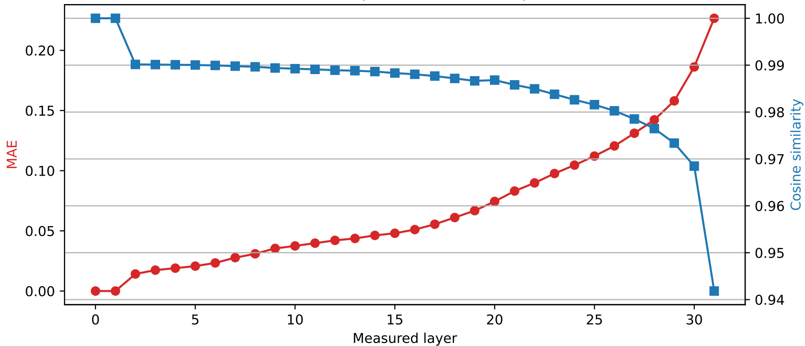
Mistral-7B-Instruct-v0.3 | Quantized layer 1 | float16 → int4
