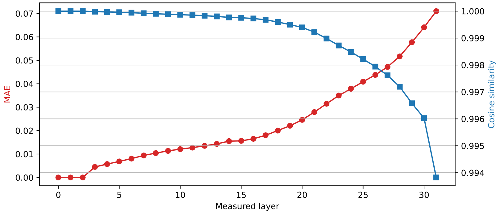
Mistral-7B-Instruct-v0.3 | Quantized layer 2 | float16 → int4
