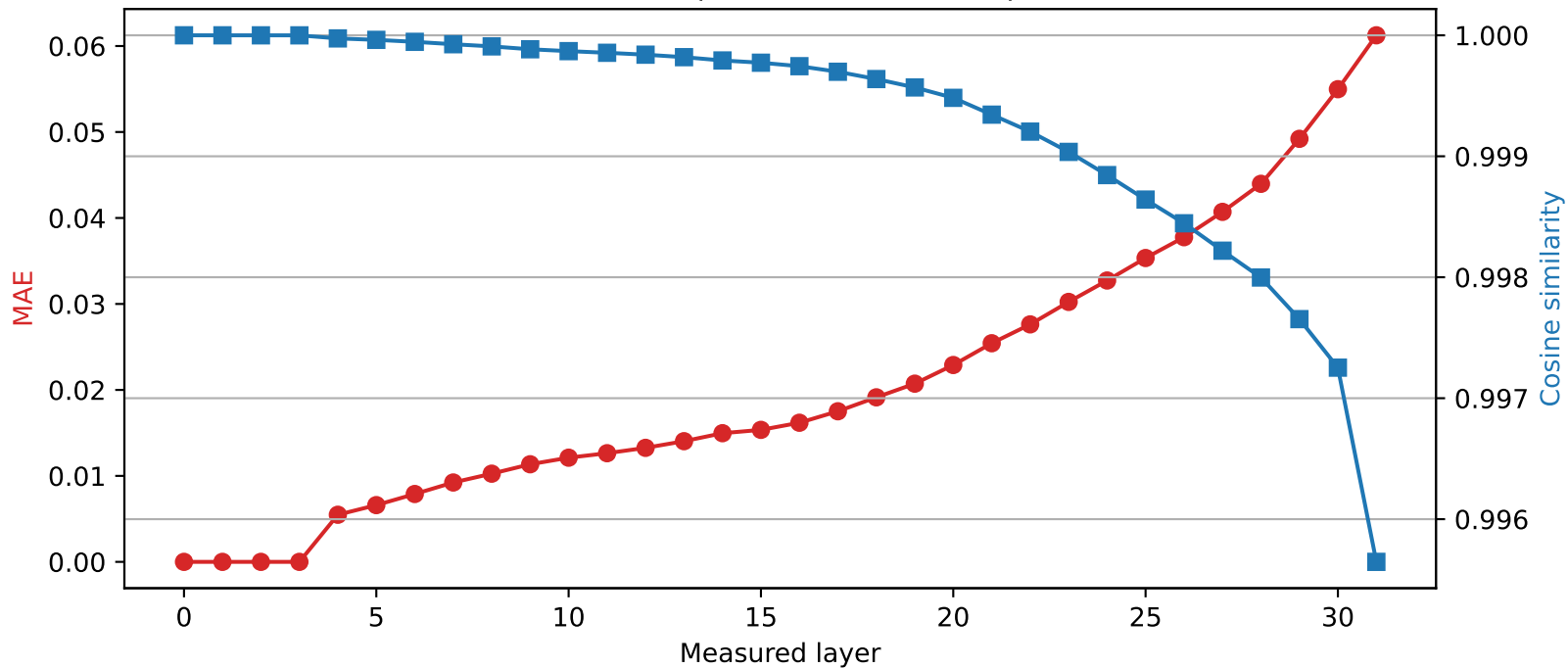
Mistral-7B-Instruct-v0.3 | Quantized layer 3 | float16 → int4
