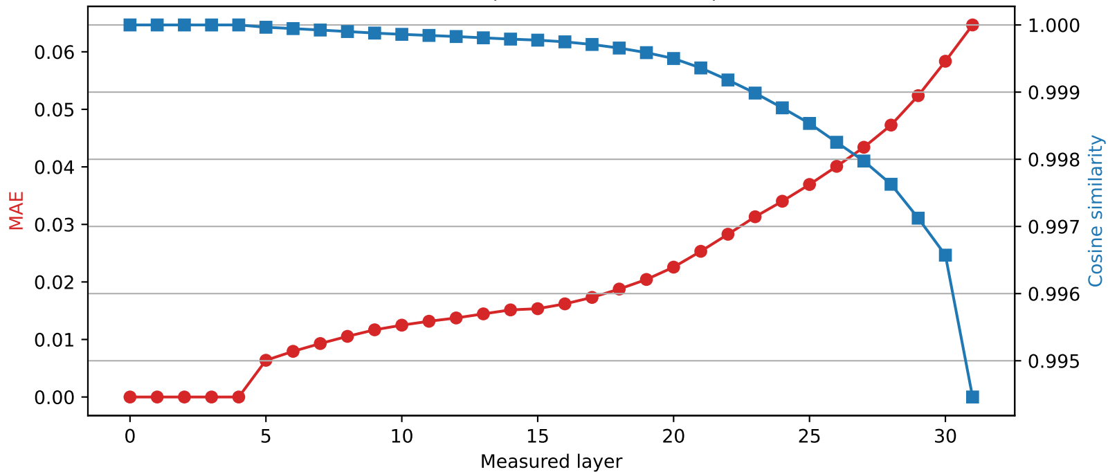
Mistral-7B-Instruct-v0.3 | Quantized layer 4 | float16 → int4
