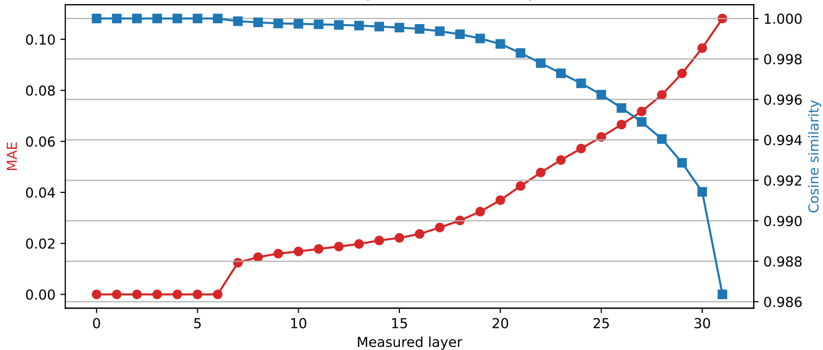
Mistral-7B-Instruct-v0.3 | Quantized layer 6 | float16 \rightarrow int4
